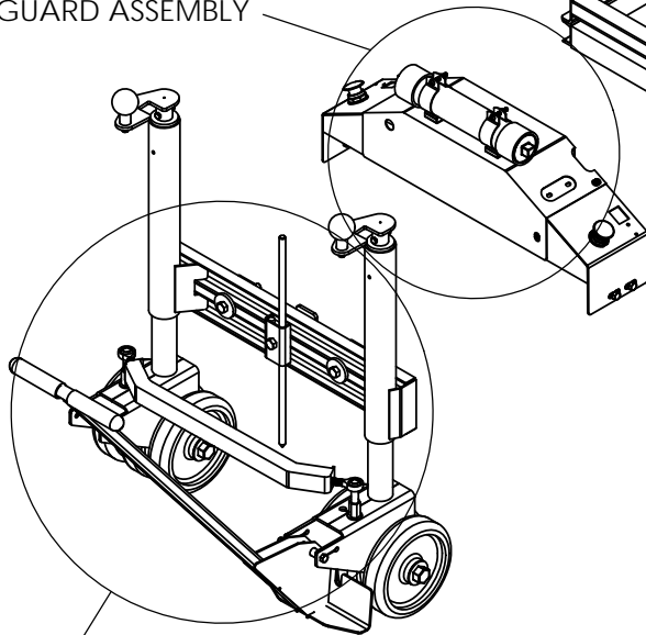
BELT GUARD ASSEMBLY
