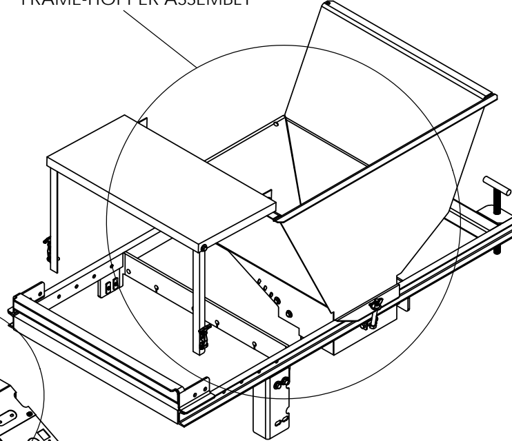
FRAME-HOPPER ASSEMBLY
